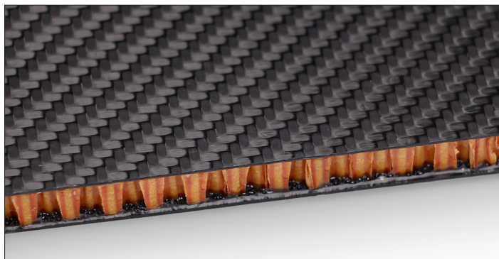
Nomex® honeycomb carbon fibre panel made using XC130 prepreg and XA120 adhesive film.
