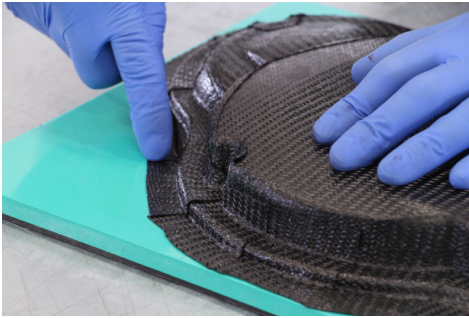
XT135 tooling prepreg being laminated onto a complex pattern in individual panels.
